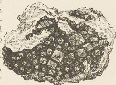
RED COPPER.
